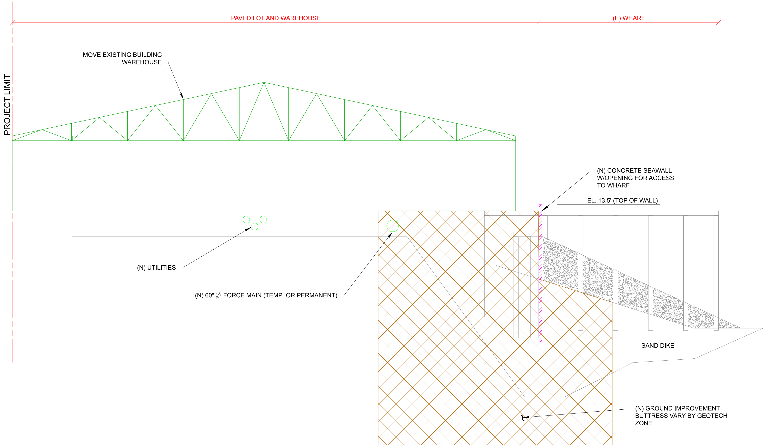
REACH 4 - SECTION 12 - PIER 80 - RECOMMENDED PLAN
