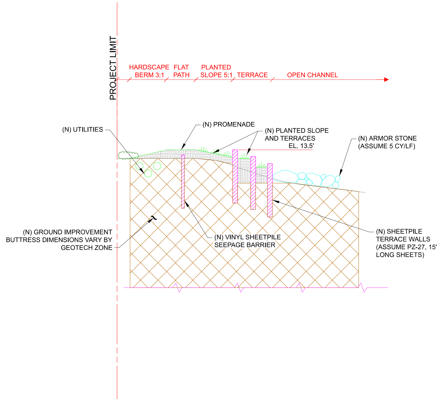
REACH 3 - SECTION 7 - MISSION CREEK NORTH - RECOMMENDED PLAN
